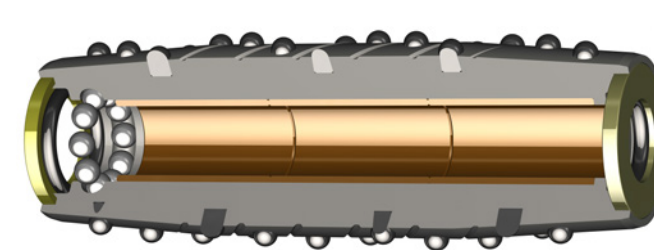
Silver plated high strength copper-nickle-tin alloy floating bearing bushings.
